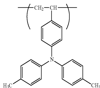
[Chemical Formula 21]
