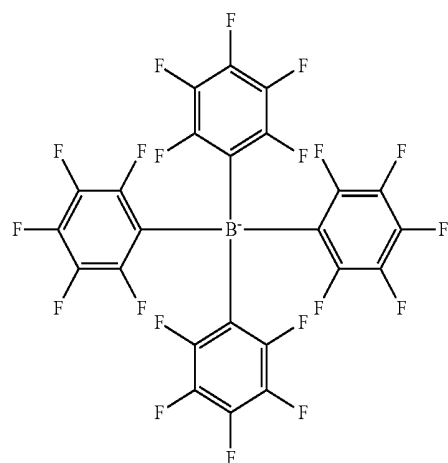
[Chemical Formula 6]
