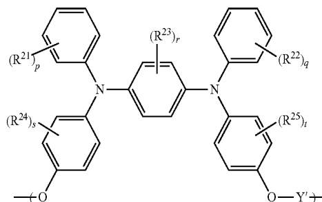
[Chemical Formula 12]
