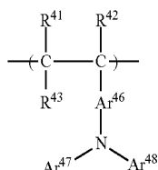
[Chemical Formula 19]
