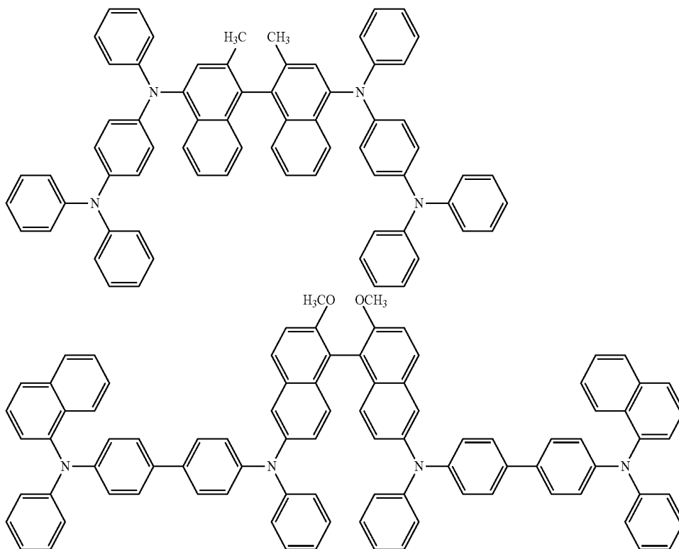
[Chemical Formula 23]
