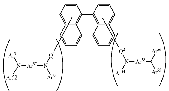
[[Chemical Formula 22]
