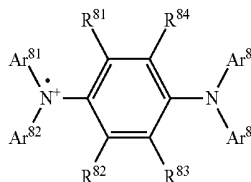
[Chemical Formula 7]
