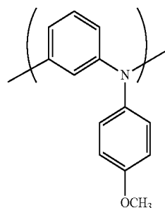
[Chemical Formula 21]
